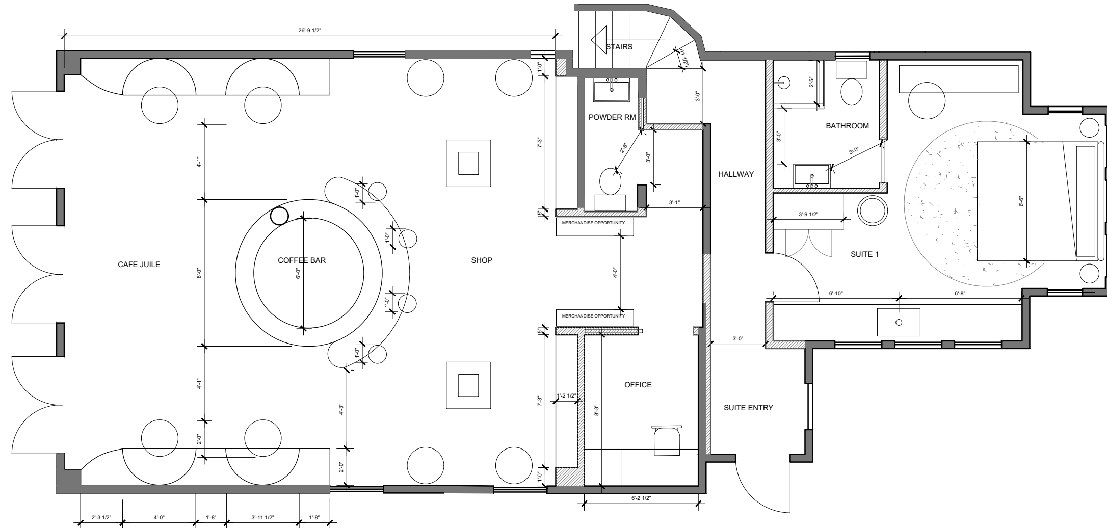
1 ID3-1 FIRST FLOOR PROPOSED FLOOR PLAN SCALE 3/16" = 1'-0"
