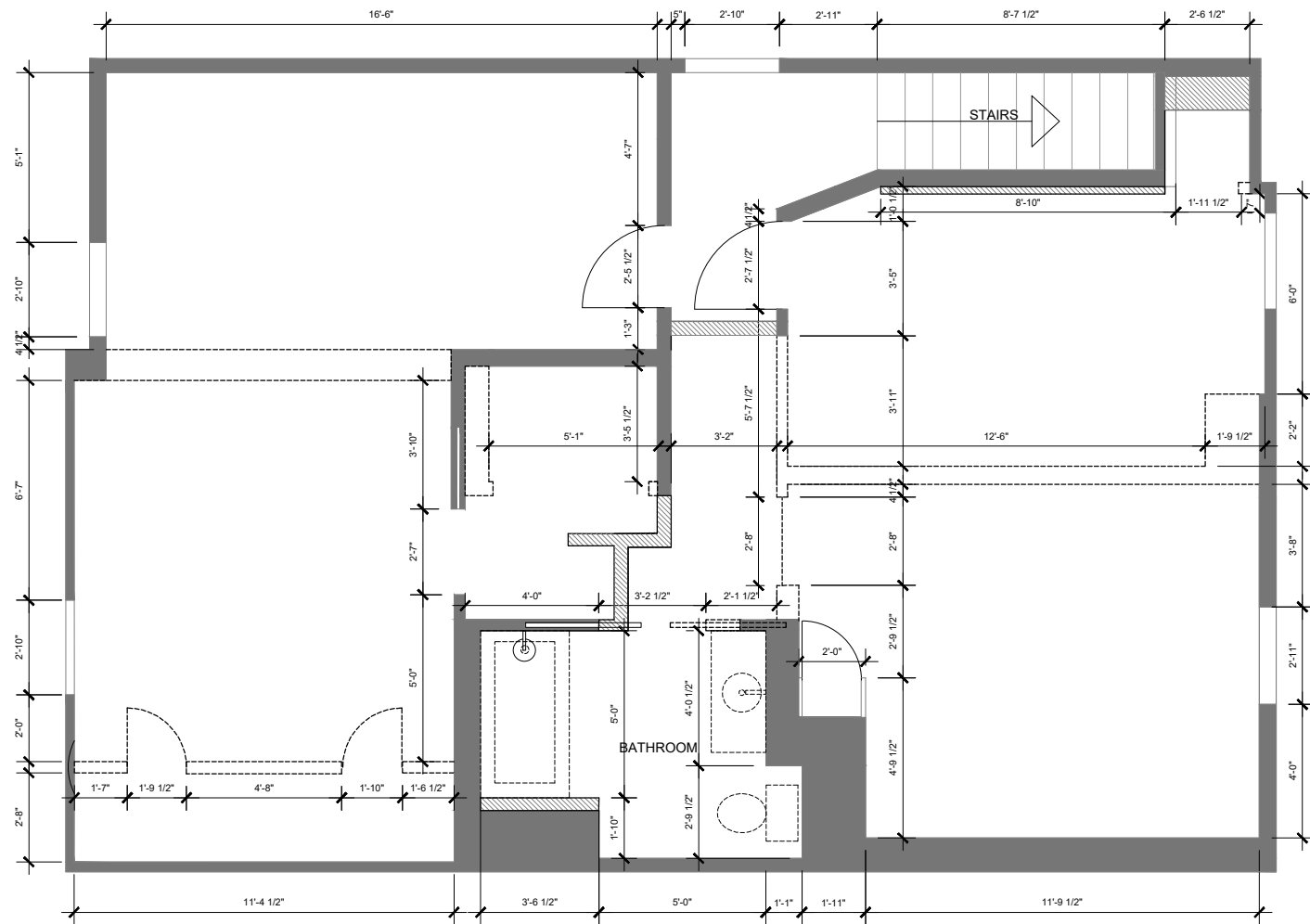
1 SECOND FLOOR AS BUILT FLOOR PLAN ID1-2 SCALE 3/16" = 1'-0"
